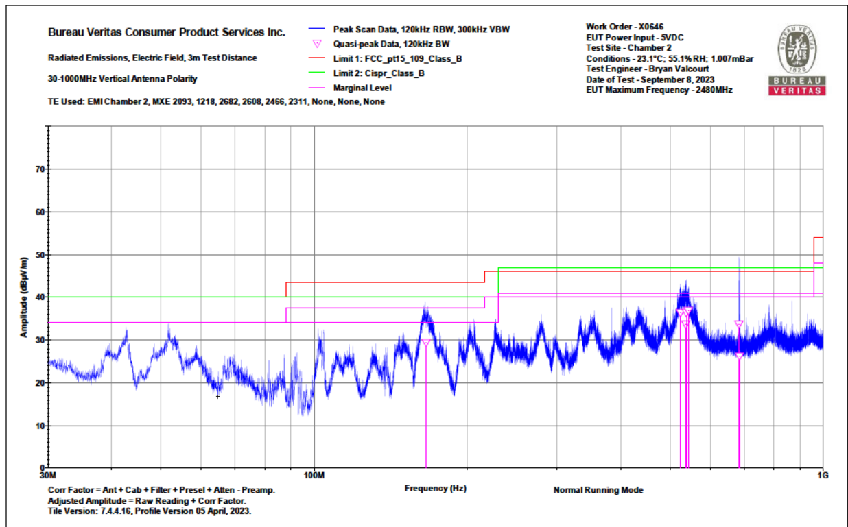
30-1000MHz FCC &amp; CISPR Vertical Graph
