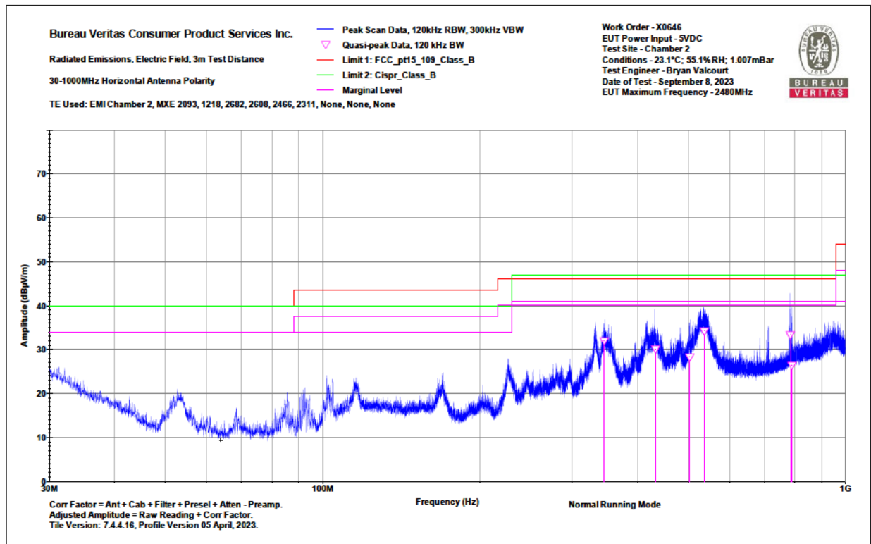
30-1000MHz FCC &amp; CISPR Horizontal Graph
