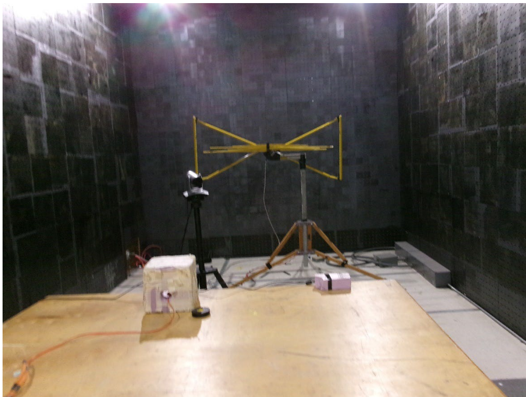
80-1000MHz Rear
